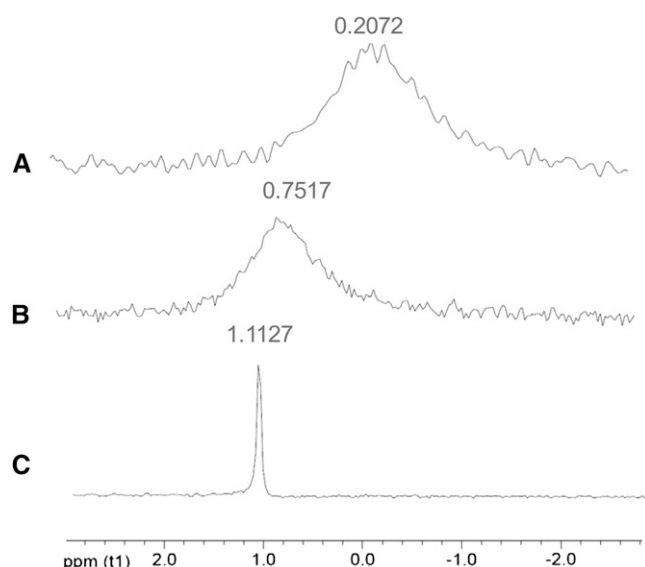
Figure 9. ^{27}\text{Al} -NMR Profile of \text{AlCl}_3 in the Presence of Citrate and Xyloglucan.
