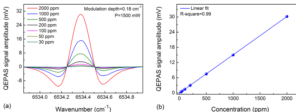
FIG. 6. QEPAS signal amplitude. (a) Different C 2 H 2 concentration levels with a modulation depth of 0.18 cm -1 . (b) QEPAS signal amplitude from Fig. 6(a) as a function of C 2 H 2 concentrations.
