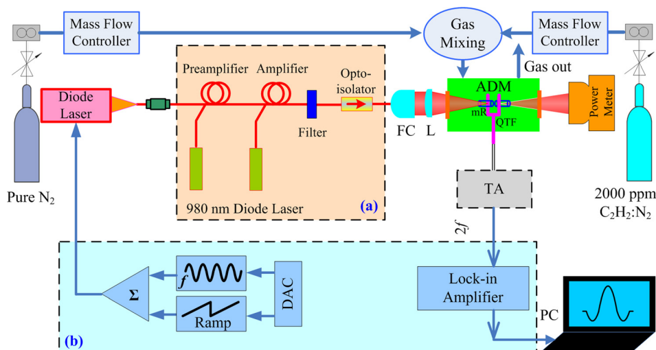
FIG. 2. Schematic of a C_2H_2 -QEPAS sensor. (a) EDFA. (b) Control electronics for modulation and demodulation. FC: fiber collimator; L: plano-convex lens; ADM: acoustic detection module; mR: micro-resonator; and TA: transimpedance amplifier.
