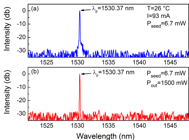
FIG. 1. Diode laser emission spectrum. (a) Seed diode laser with a 6.7 mW output power. (b) EDFA amplified diode laser with a 1500 mW output power.
