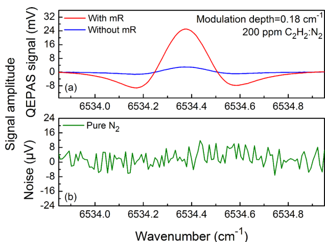
FIG. 7. Signal amplitude. (a) QEPAS signal with and without a mR. (b) Pure N 2 for a noise background determination. mR: micro-resonator.
