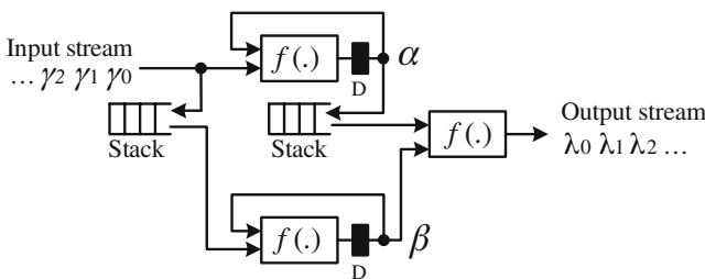
Figure 13 MAP processor structure for single parity check code.
