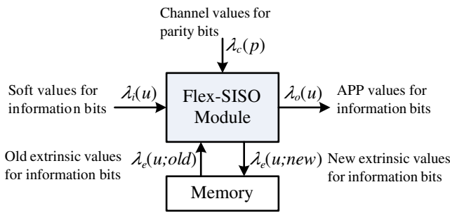
Figure 4 Flex-SISO module.
