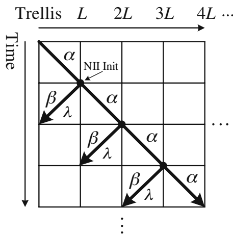
Figure 20 Data flow graph for Turbo decoding.
