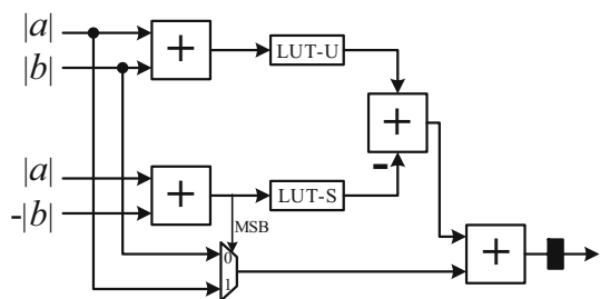
Figure 14 Circuit diagram for the LDPC |f(a, b)| functional unit.
