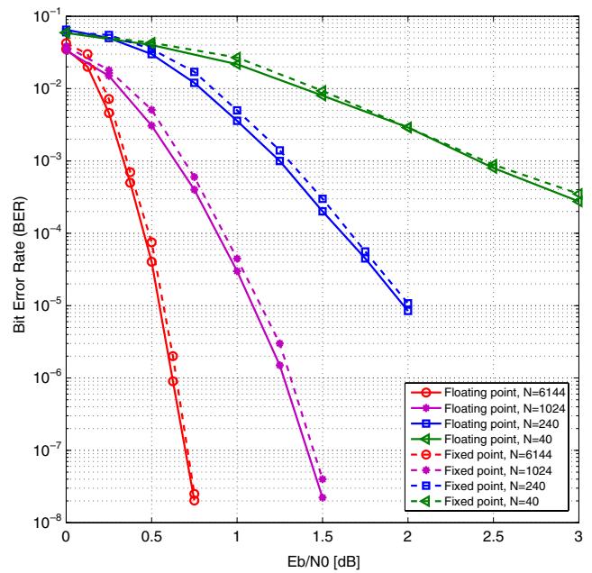
Figure 18 Simulation results for 3GPP-LTE Turbo codes with a variety of block sizes.
