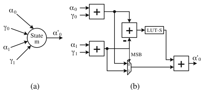
Figure 10 Turbo ACSA structure. a Flow of state metric calculation. b Circuit diagram for the Turbo ACSA unit.
