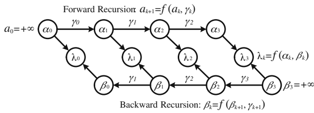
Figure 12 A forward–backward decoding flow to compute the extrinsic LLRs for single parity check code.
