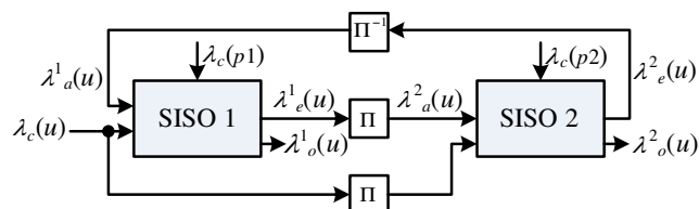
Figure 7 Traditional Turbo decoding procedure using two SISO decoders, where the extrinsic LLR values are exchanged between two SISO decoders.
