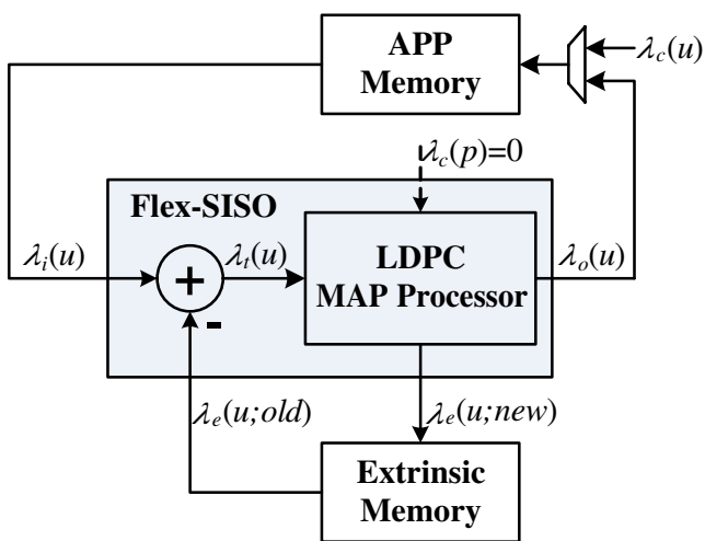
Figure 6 LDPC decoder architecture based on the Flex-SISO module.
