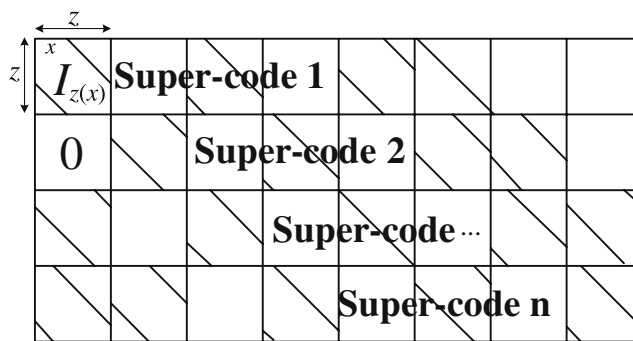
Figure 3 A block-structured parity check matrix, where each block row (or layer) defines a super-code. Each sub-matrix of the parity check matrix is either a zero matrix or a z \times z cyclically shifted identity matrix.
