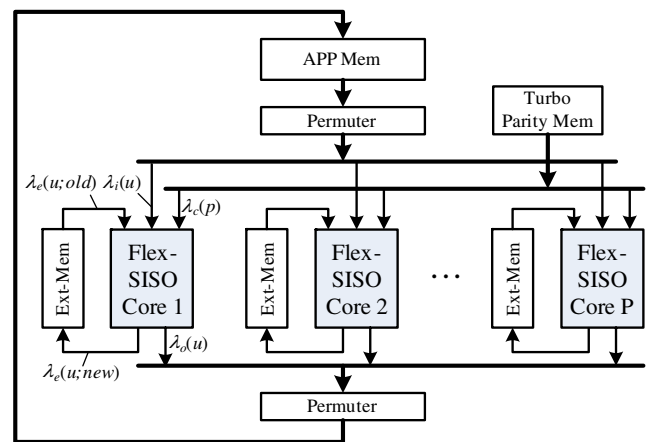
Figure 22 Parallel LDPC/Turbo decoder architecture based on multiple Flex-SISO decoder cores.
