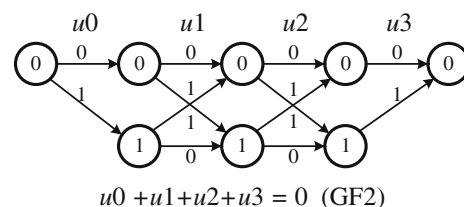
Figure 11 Trellis structure for a single parity check code.
