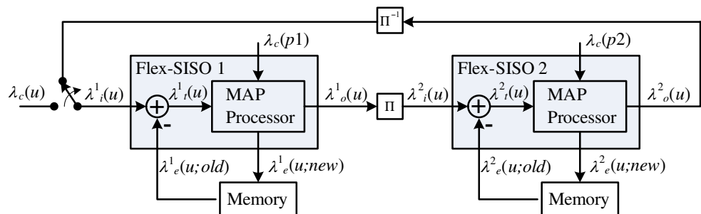
Figure 8 Modified Turbo decoding procedure using two Flex-SISO modules. The soft LLR values are exchanged between two SISO modules.
