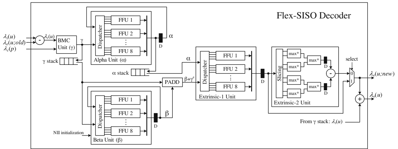
Figure 19 Flexible SISO decoder architecture.
