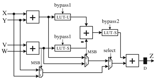
Figure 15 Circuit diagram for the flexible functional unit (FFU) for LDPC/Turbo decoding.
