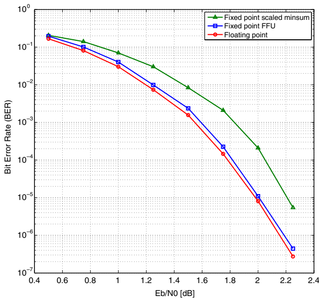
Figure 16 Simulation results for a rate 1/2, length 2304 WiMAX LDPC code.
