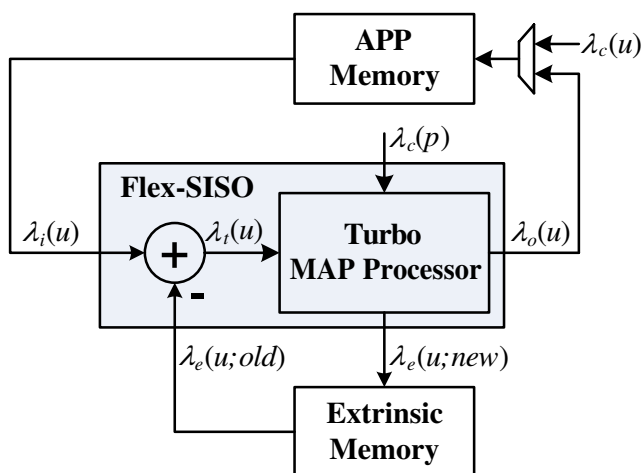
Figure 9 Turbo decoder architecture based on the Flex-SISO module.
