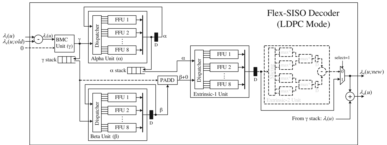
Figure 21 Flexible SISO decoder architecture in LDPC mode.
