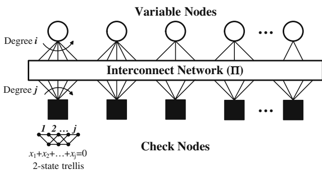
Figure 1 Trellis representation for LDPC codes where a two-state trellis diagram is associated with each check node.
