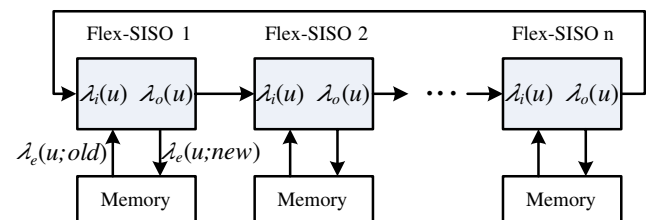
Figure 5 LDPC decoding using Flex-SISO modules where a LDPC code is decomposed into n super-codes, and n Flex-SISO modules are connected in series to decode.
