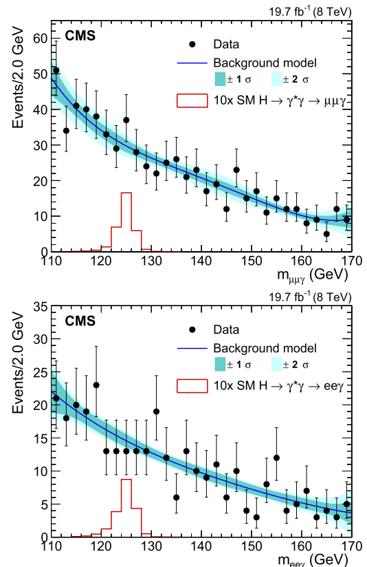
Fig. 4. The m_{\mu\mu\gamma} (top) and m_{ee\gamma} (bottom) spectra for 8 TeV data (points with error bars), together with the result of a background-only fit to the data. The 1\sigma and 2\sigma uncertainty bands represent the uncertainty in the parameters of the fitted function. The expected contribution from the SM Higgs boson signal with m_H = 125 \text{ GeV} , scaled up by a factor of 10, is shown as a histogram.
